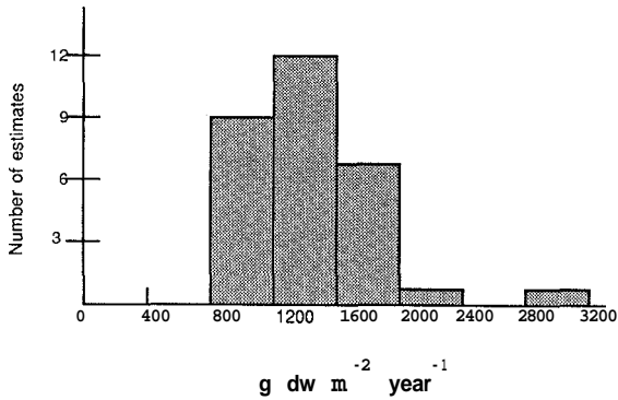
Fig. 1. Distribution of annual primary production rates in the Turew landscape (after Ryszkowski, in press).
