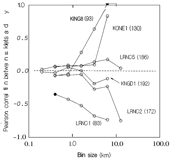
Fig. 2. Scale-dependence of the spatial correlation between auklets and their prey across the six transects. The scale on the horizontal axis reflects the distance over which data were lumped for analysis. Correlations were computed with data at the most finely resolved spatial scale, then adjacent bins of data were combined into double-sized bins and correlations were recomputed, then adjacent double-sized bins of data were combined into quadruple-sized bins and correlations were recomputed, etc. Sample sizes for correlations computed at the finest scale are shown; sample sizes for broader-scale correlations are successively halved. For comparative purposes, statistically significant correlations (adjusted for a type I family-wide error rate of p = 0.05 ) are indicated on the figure by filled circles. Note, however, that statistical significance is likely to be inflated by the lack of independence in spatially dependent data, so 'significance' should be interpreted cautiously.
