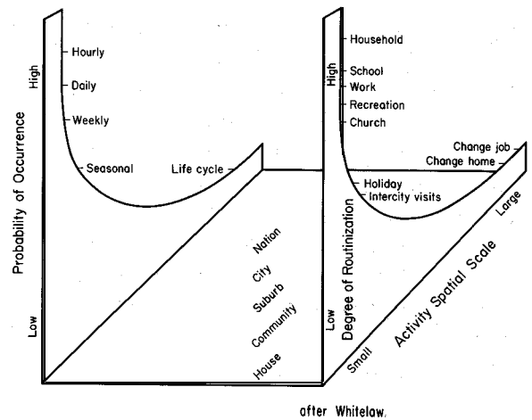
Fig. 1. The activity space of individuals as it relates to time involved, distance travelled, degree of routinization, and probability of occurrence.
