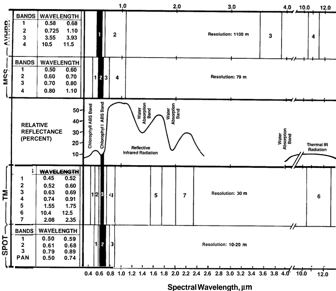
Fig. 1. Spectral and spatial resolution for four common satellite sensors: AVHRR, MSS, TM and SPOT. Also shown is a spectral response curve for typical green vegetation.
