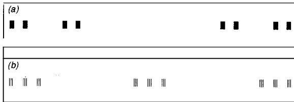
Fig. 1. Cantor dusts. The fractal dimension D of the dusts equals \ln N / \ln(1/r) , where N is the number of smaller pieces generated and r is the size reduction at each iteration (Mandelbrot 1983; Feder 1988). Each dust is shown after 3 iterations. A: N = 2 and r = 1/4 . B: N = 3 and r = 1/9 . Both dusts have a D of 0.5. The differences in appearance or texture are measured by their lacunarity.
