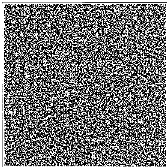
Fig. 5. 'Bottom' map, p_1 = p_2 = 1 and p_3 = \mathbf{P} = 0.5 .
