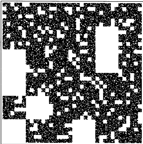
Fig. 4. 'Same' map. This map and those in figures 5–7 are 216 \times 216 hierarchical maps (Table 2). For this map \mathbf{P} equals 0.522 and p_1 = p_2 = p_3 = 0.806 .
