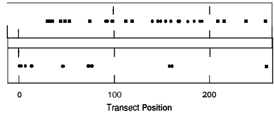
Fig. 11. Two simulated 258 point transects, with 33 occurrences of habitat or organism of interest. A: Randomly distributed points. B: A random fractal series of points. This series is a Lhy dust, which is a randomized version of the Cantor dusts in Fig. 1 and has a fractal dimension of 0.8 (Mandelbrot 19983, Voss 1988). Notice the clumping of points.
