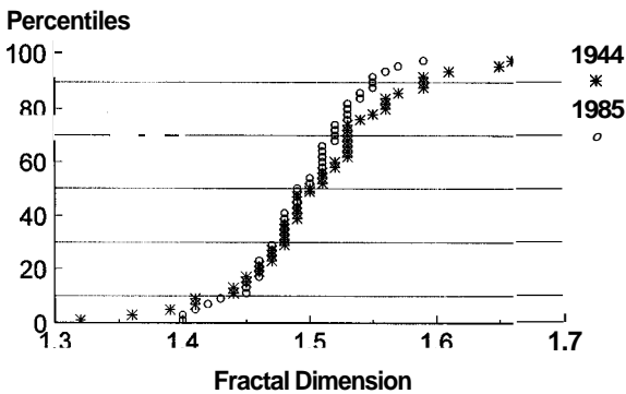
Fig. 6. Percentile plots of index D (fractal dimension) for 1944 and 1985.
