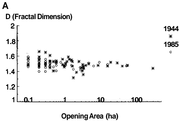
Fig. 5. Size of openings vs. A) index D and B) index C.
