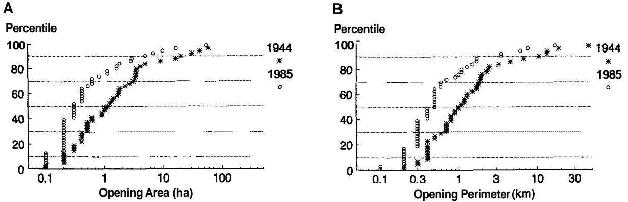
Fig. 1. Percentile plots of A) area and B) perimeter of openings illustrating how the openings on the 1944 aerial photographs tend to be larger than those found on the 1985 aerial photographs.
