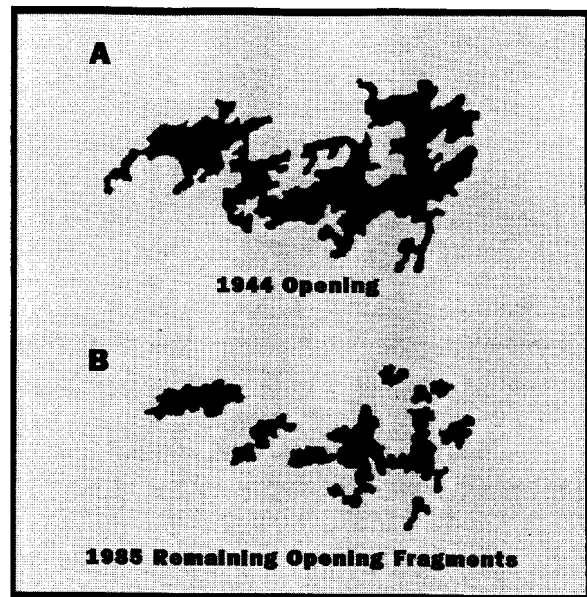
Fig. 7. Schematic representation of general pattern of fragmentation and shrinking of openings from A) 1944 to B) 1985.
