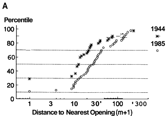
Fig. 3. Percentil plots illustrating increases between 1944 and 1985 in A) distance to nearest openings ( m+1 necessary because log of 0 is undefined) and B) distance between nearest neighbor pair for each sample point.
