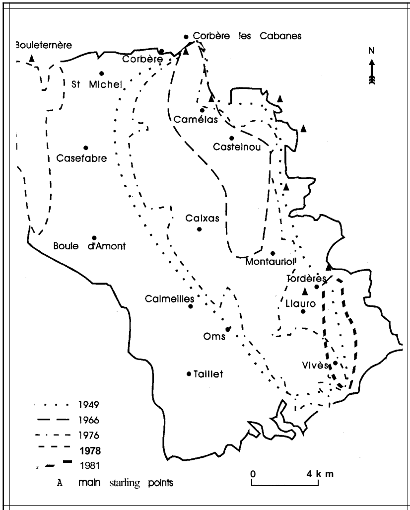
Fig. 1. Locations and areas of the last major wildfires in the Massif des Aspès (from Amigo 1981).
